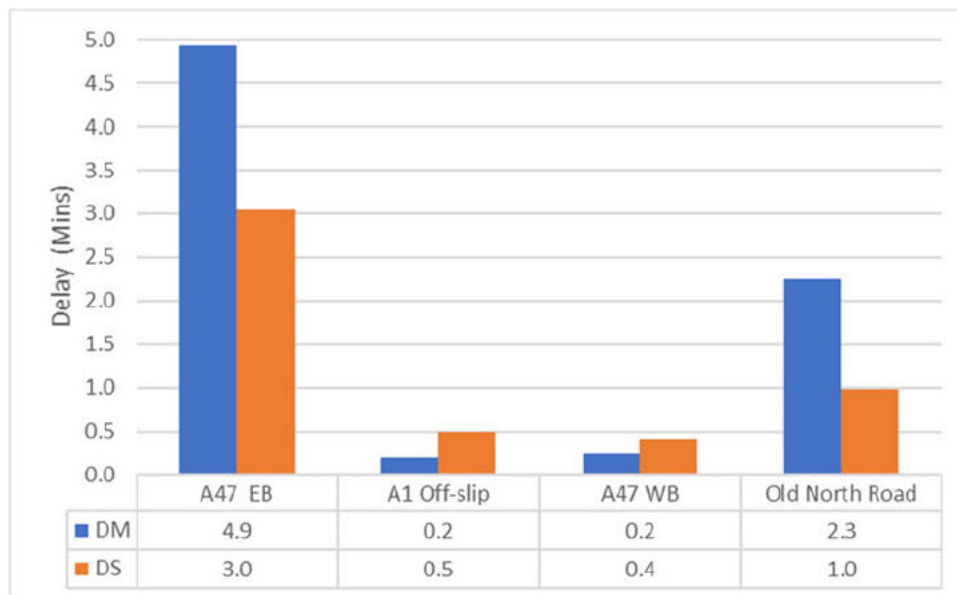
Figure 7-11: Wansford West roundabout AM peak – average vehicle delay
